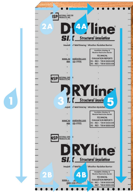
Figure 9. Installation, Step 3
