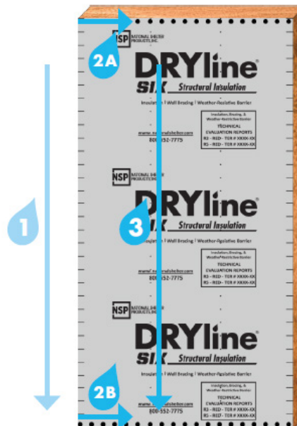
Figure 8. Installation, Step 2
