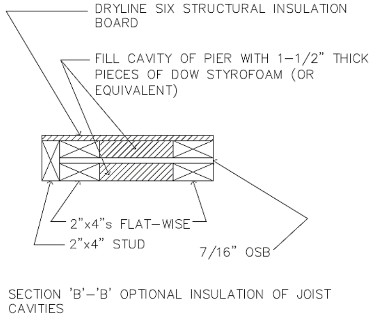
Figure 6. DRYline® SIX Structural Insulation Board 12" to 24" PFH Section B-B (Portal Pier Assembly)
