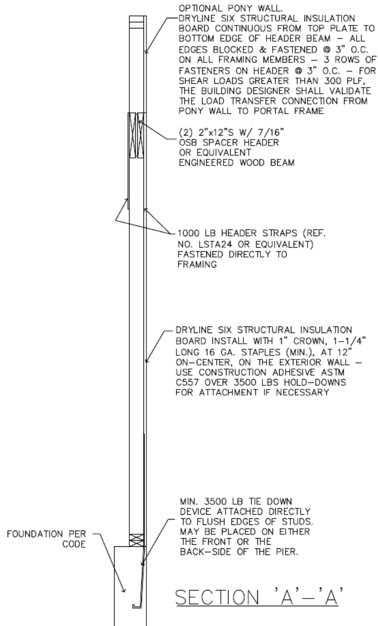
Figure 5. DRYline® SIX Structural Insulation Board 12" to 24" PFH Section A-A
