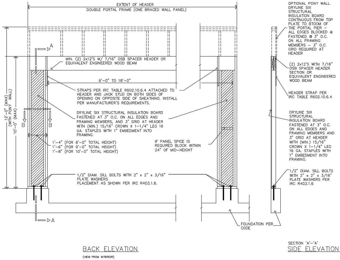
Figure 2. DRYline® SIX Structural Insulation Board Structural Sheathing CS-PF
