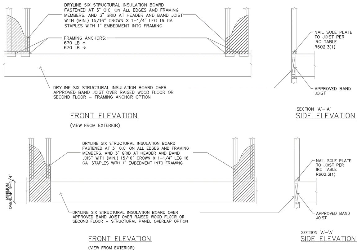
Figure 3. DRYline® SIX Structural Insulation Board Structural Sheathing CS-PF (Anchorage Details)
