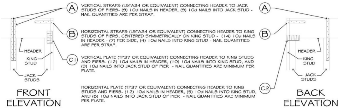
Figure 4. Construction Details of DRYline® SIX Structural Insulation Board 12" to 24" PFH
